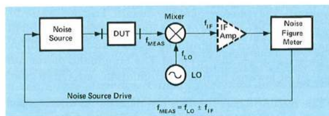
Figure 2-2. The general block diagram of a down converter to be used as part of a noise figure measurement system. The IF amplifier is outlined in dashes because the high sensitivity of the 8970A Noise Figure Meter means the IF amplifier is usually not necessary. The 8970A, because of its tunable input frequency or variable IF, allows swept frequency measurements with a fixed-frequency local oscillator.
