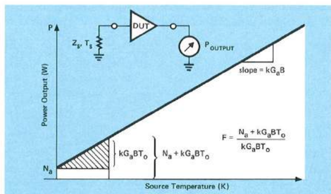
Figure 1-4. Noise figure shows the behavior at standard temperature T_0 ( \approx 290 K). Noise figure is the ratio of the total power output ( N_a + kT_0 BG_a ) to that portion that is due to the amplified input noise power ( kT_0 BG_a ). Noise figure is usually expressed in dB.
