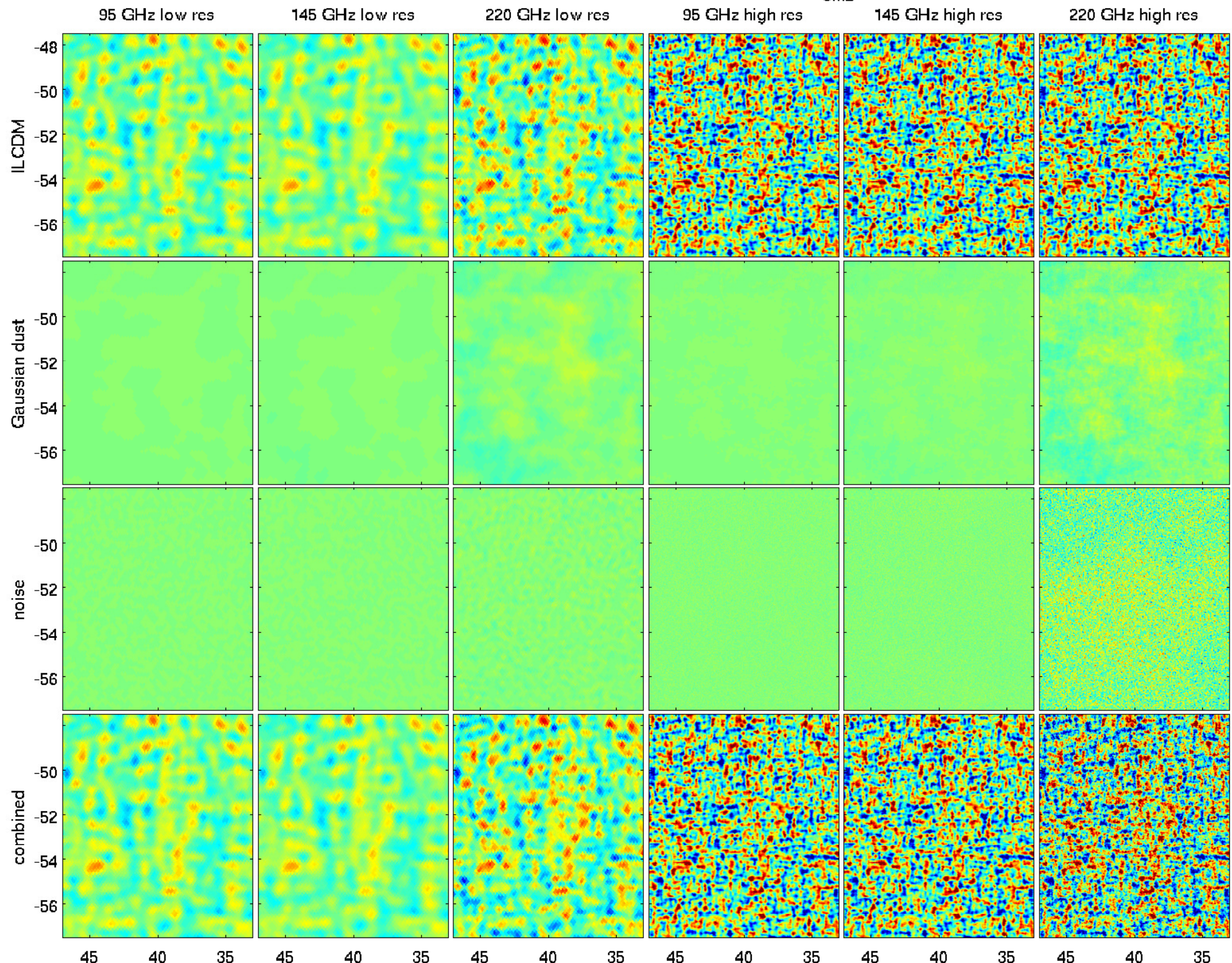
06b.00 realization 0000 Q maps (all colorstretch \pm 10\mu_{\text{CMB}}\text{K} )
